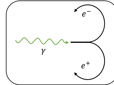
Pair production – an electron-positron pair produced a proton-antiproton pair
